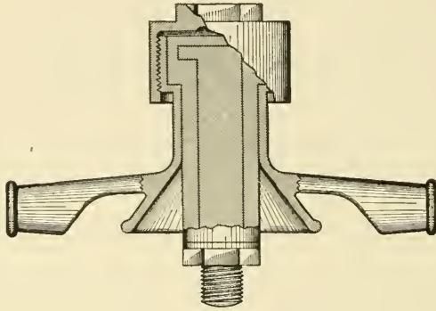
Fig. 183. Section of a Hanger
